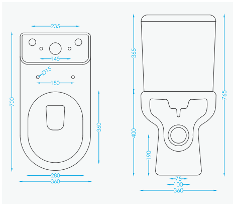
SOFIA (P Trap) Water Closet with Soft Close Seat Water Tank with Dual Flushing Unit. Two Piece WC (L700 W360 H765)
